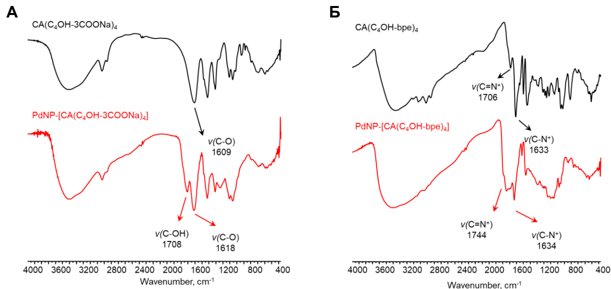
Рисунок 4.2 – ИК-спектры (А) \text{CA}(\text{C}_4\text{OH-3COONa})_4 , \text{PdNP-}[\text{CA}(\text{C}_4\text{OH-3COONa})_4] ; (Б) \text{CA}(\text{C}_4\text{OH-bpe})_4 , \text{PdNP-}[\text{CA}(\text{C}_4\text{OH-bpe})_4] в KBr
