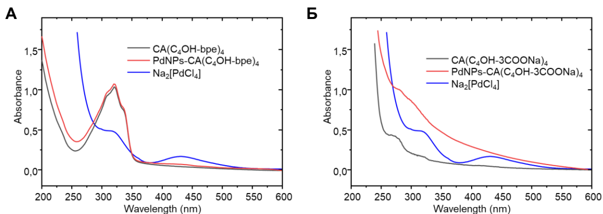
Рисунок 4.1 – УФ спектры (А) \text{CA}(\text{C}_4\text{OH-bpe})_4 , \text{PdNP-}[\text{CA}(\text{C}_4\text{OH-bpe})_4] и \text{Na}_2[\text{PdCl}_4] ; (Б) \text{CA}(\text{C}_4\text{OH-3COONa})_4 , \text{PdNP-}[\text{CA}(\text{C}_4\text{OH-3COONa})_4] и \text{Na}_2[\text{PdCl}_4] ; C[\text{Pd}] = 0,05 \text{ mM} , C(\text{CA}) = 0,01 \text{ mM} , \text{H}_2\text{O} , 25^\circ\text{C}
